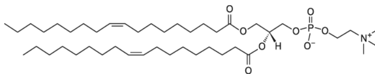
Fig. 2. Molecular structure of DOPC (1,2-dioleoyl- sn -glycero-3-phosphocholine).
