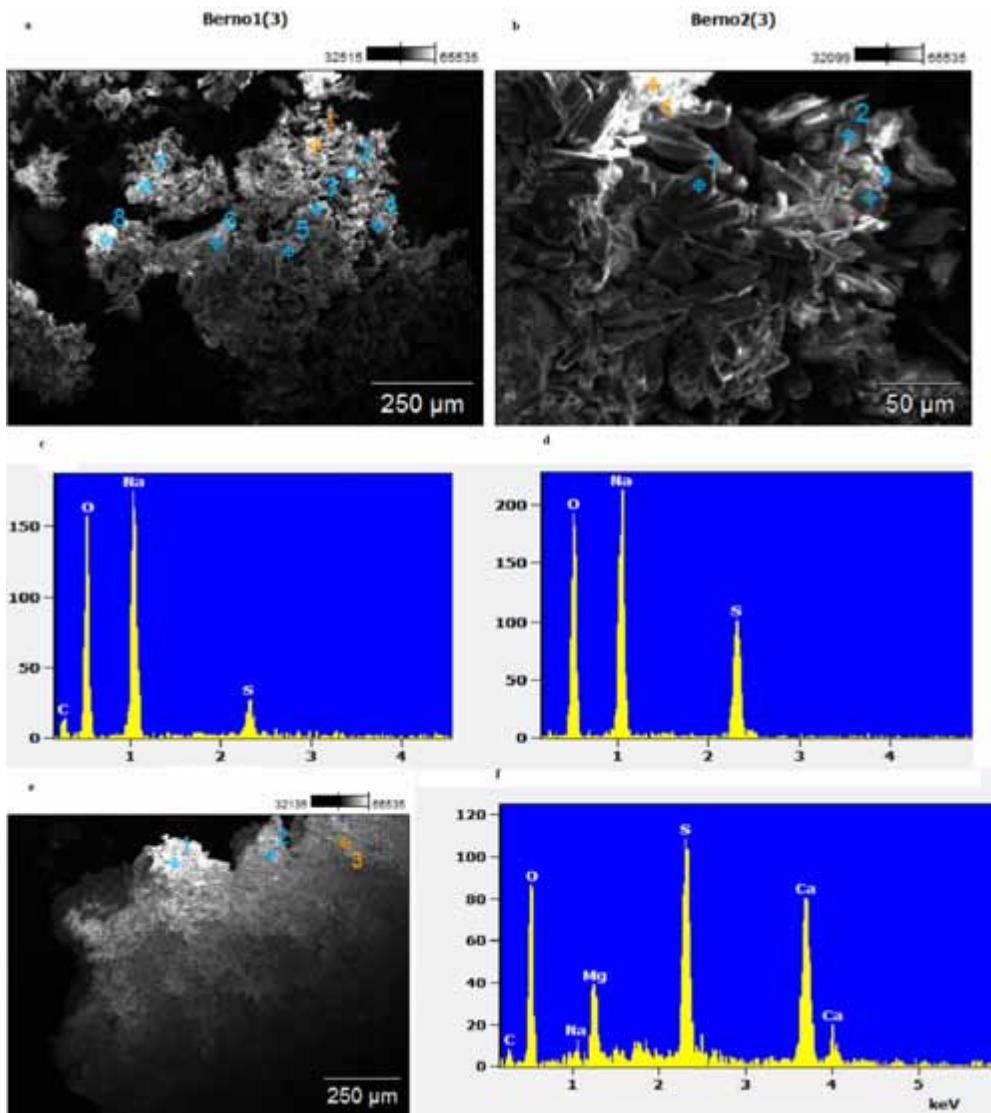
Figure 3: BSE microphotographs of mirabilite (a,b,c,d) and gipsum (e,f) with EDS spectra.
