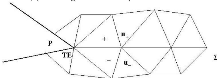
Fig. 2. The Kutta-Zhukovsky condition on slit Σ
