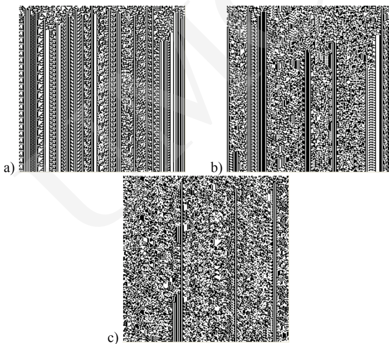
Fig. 3. Time Space Diagrams of CA run with the use of bad sets of rules: set {105, 86, 30} (a), set {86, 150, 1755030679, 1778009733, 869020563} (b) and set {105, 1720884581, 2036803240, 150, 1778009733} (c)
