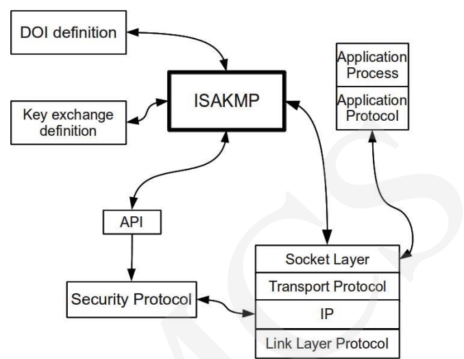
Fig. 1. ISAKMP architecture.
