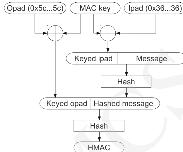
Fig. 11. HMAC calculation.
